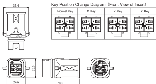
Tab Housing
