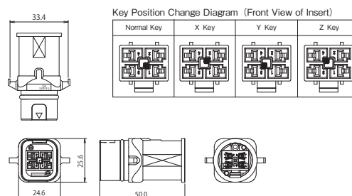
Receptacle Housing
