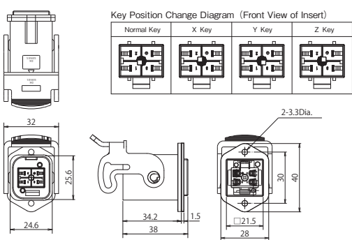
Tab Housing
