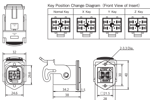
Tab Housing
