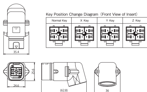
Tab Housing
