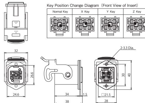
Receptacle Housing
