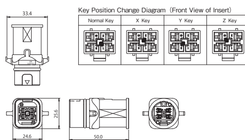
Receptacle Housing
