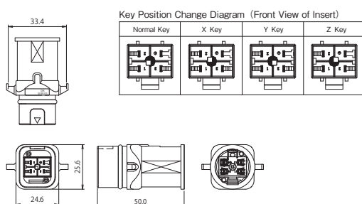
Tab Housing
