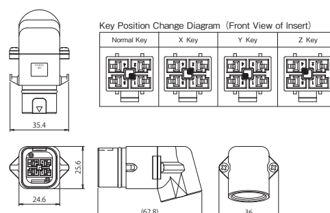
Receptacle Housing
