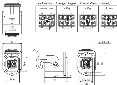
Receptacle Housing
