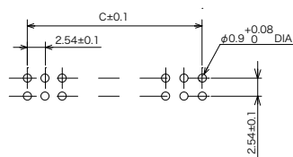
PCB Mounting Dimensions
