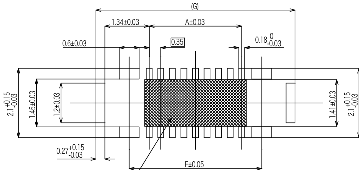
Reference P.C.B Layout (Connector Mounting Side View)
