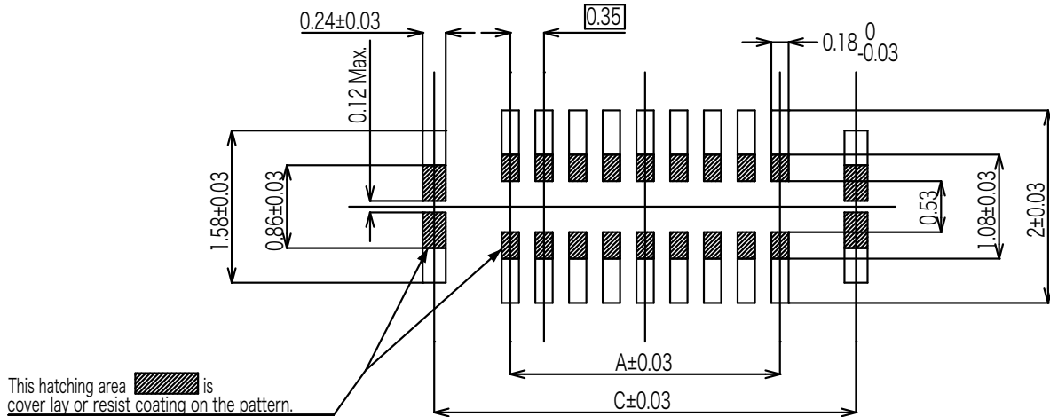
Reference P.C.B Layout (Connector Mounting Side View)
