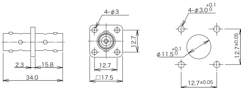
Panel Mounting Dimensions
