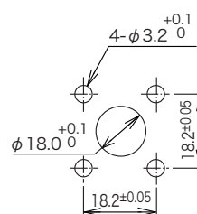
Panel Mounting Dimensions
