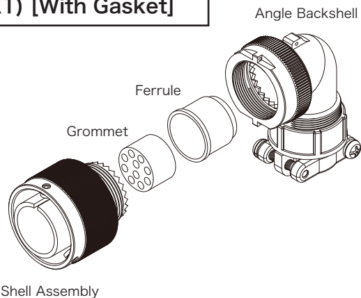
Plug Shell Assembly
